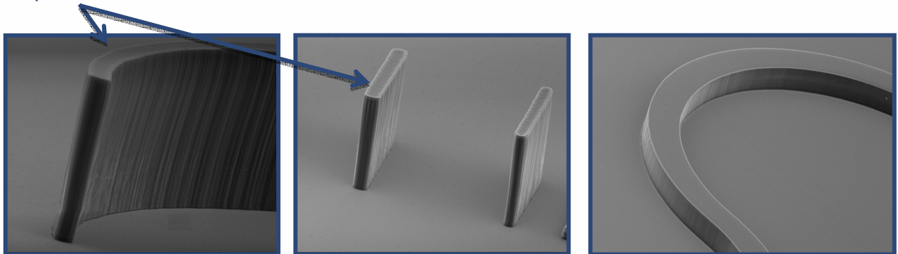
High aspect ratio photoresist lines patterned using MicroStencil emulsion glass plate
